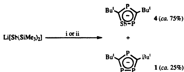
Scheme 1. Reagents and conditions: (i) \text{P}\equiv\text{C}'\text{Bu} , DME, 25°C, 72 h; (ii) (\text{Me}_3\text{Si})\text{P}=\text{C}'\text{Bu}(\text{OSiMe}_3) , DME, 25°C, 72 h.
